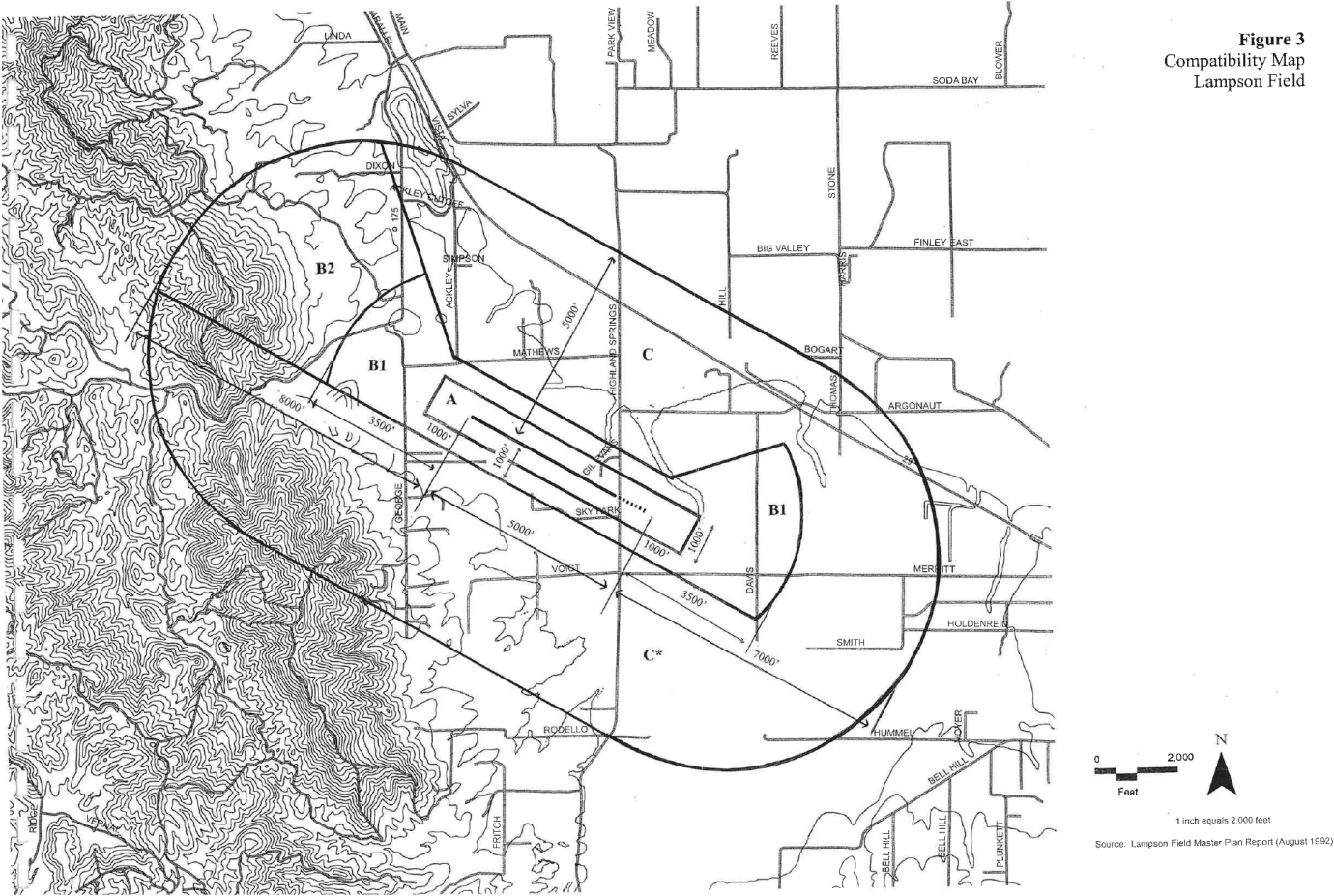
Figure K-10 Lampson Field Airport Compatibility Zones
