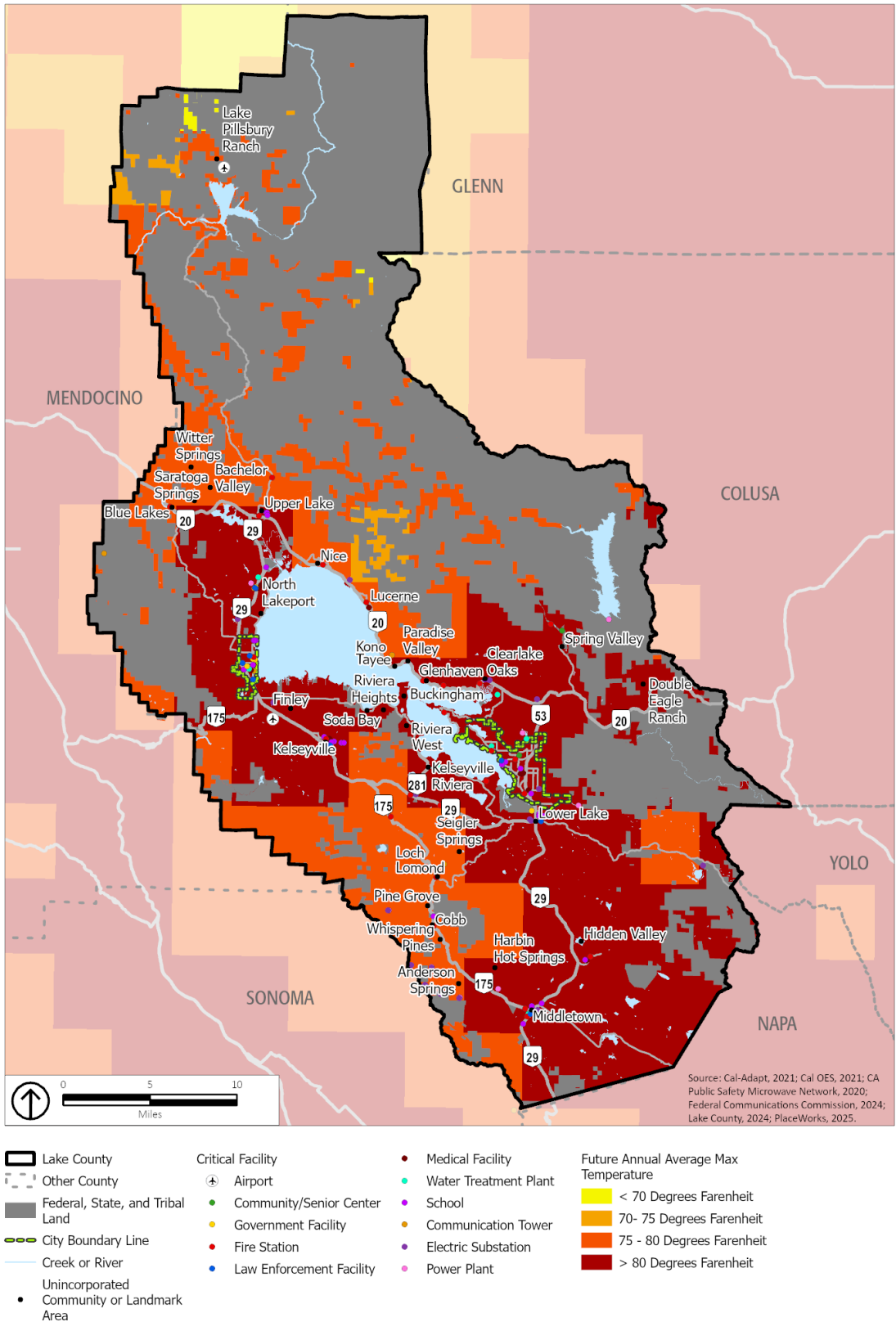
Figure D-4 Projected Annual Average High Temperatures (Late Century)
