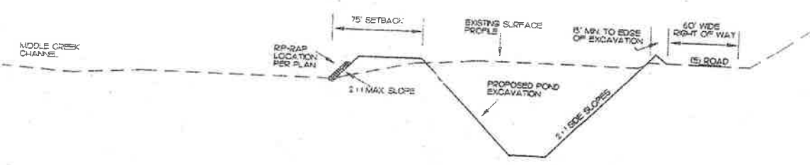
TYPICAL SECTION "A" - "A" SCALE: 1" = 50' HORIZ. 1" = 25' VERT.
