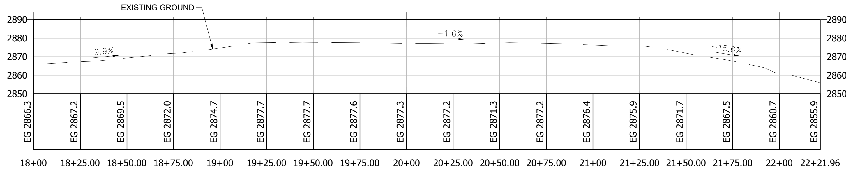
EXISTING ROAD PROFILE VIEW VERTICAL AND HORIZONTAL SCALE: 1"=30' STA: 18+00.00 TO 22+21.96
