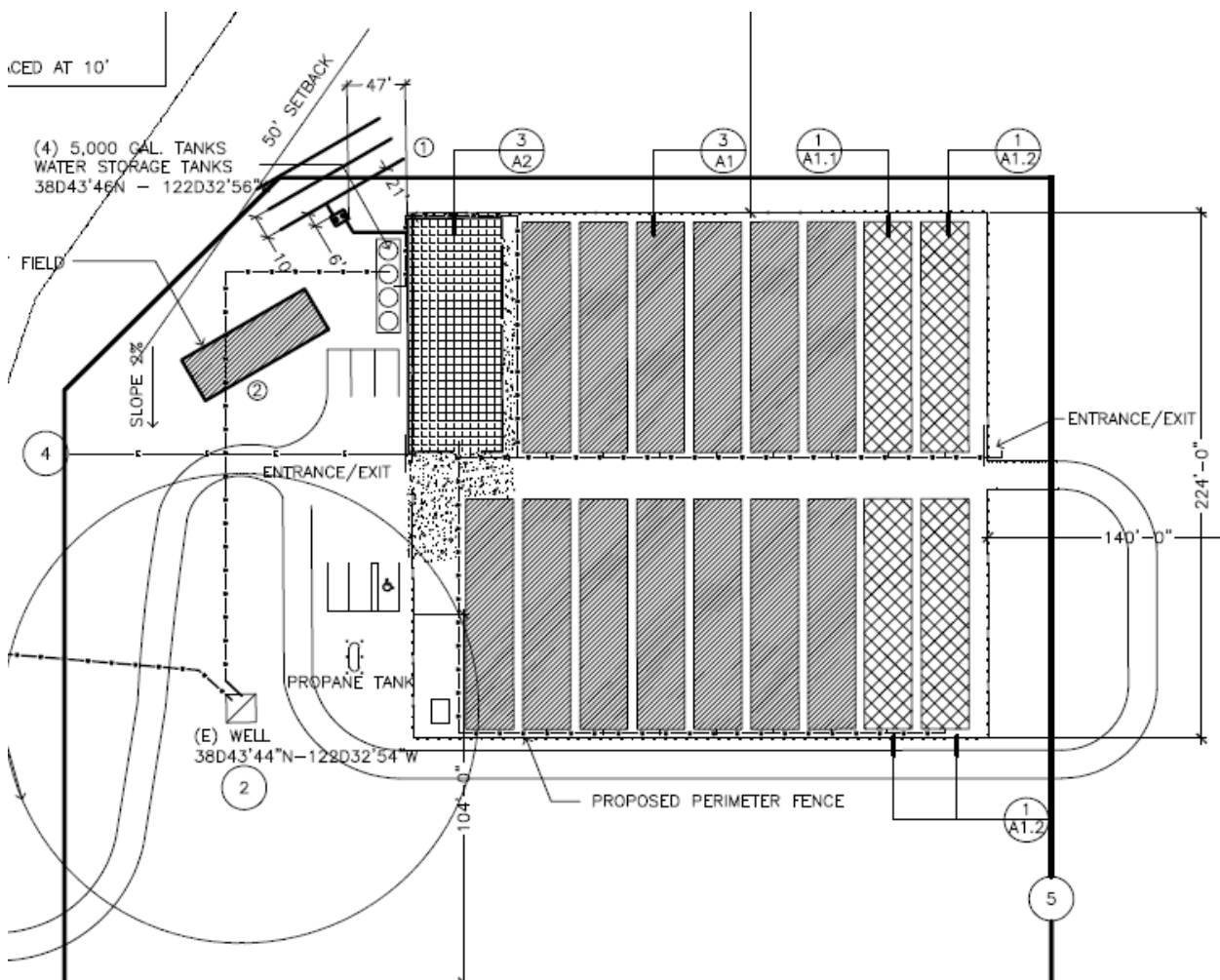
Existing and Proposed Greenhouse Locations (Attachment 5)
